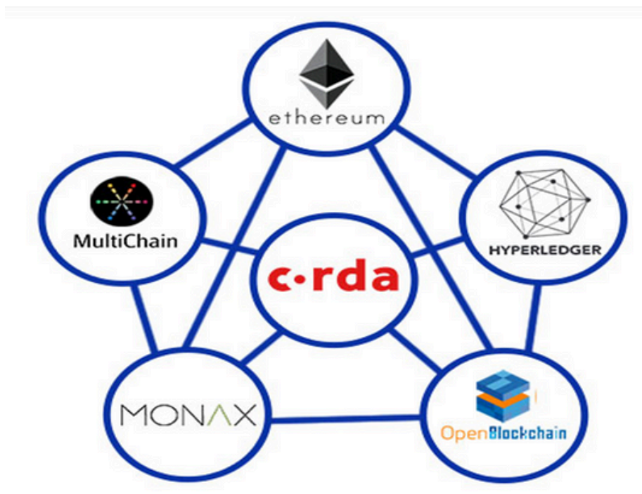
Figure 5: Blockchain Frameworks
